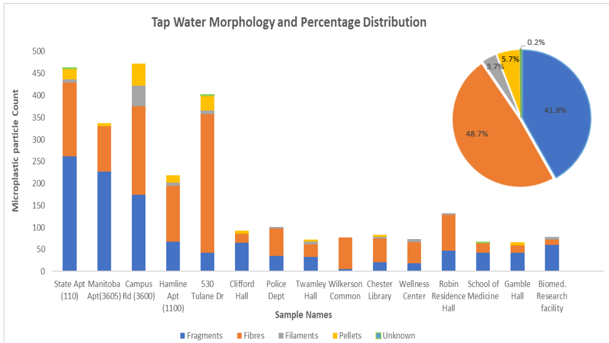
Figure 9: The percentage distribution of particles by morphology in tap water samples
